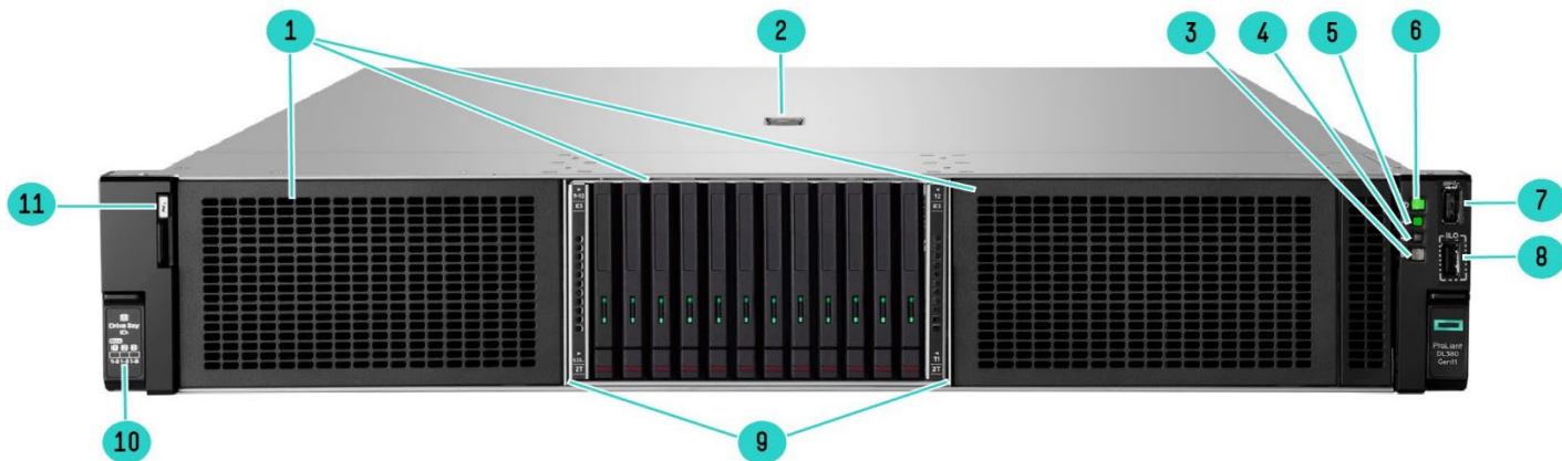
Front View –12EDSFF chassis shown
